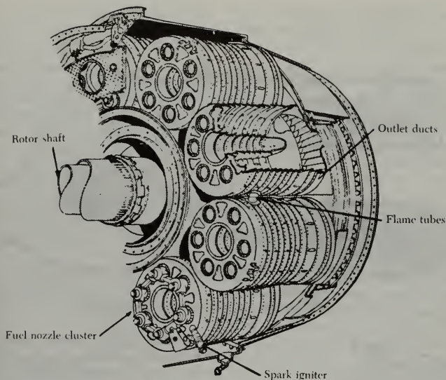
FIGURE 1-48. Can-annular combustion chamber components and arrangement.
